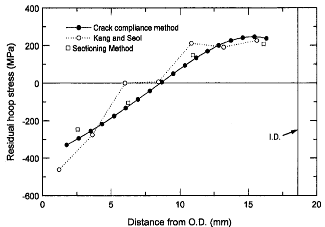
Fig. 1(a) Residual stresses predicted by Kang and Seol and their validation using sectioning procedures compared with the prediction of our crack compliance method using their strain measurements
